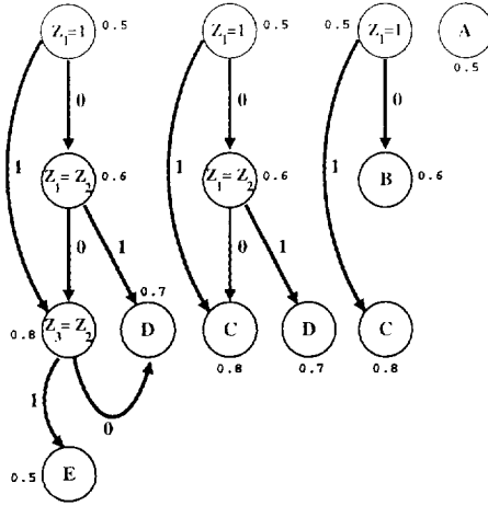
Figure 5: A decision graph and its possible prunings.
