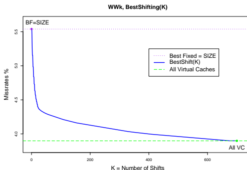
Figure 2: Optimal offline comparators. AllVC = \lim_{K \rightarrow \infty} \text{BestShifting}(K) .
